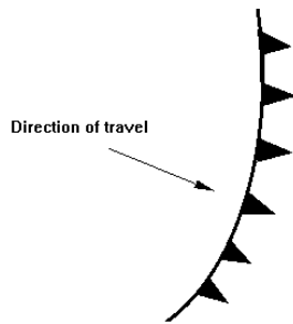
Figure 4 Cold front symbol
