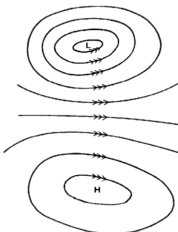
Figure 29 Rotation round pressure systems
