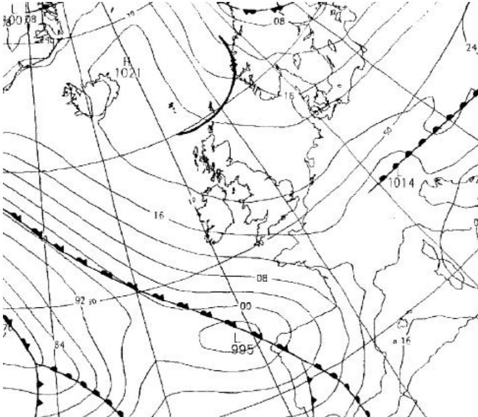
Figure 28 Synoptic chart
