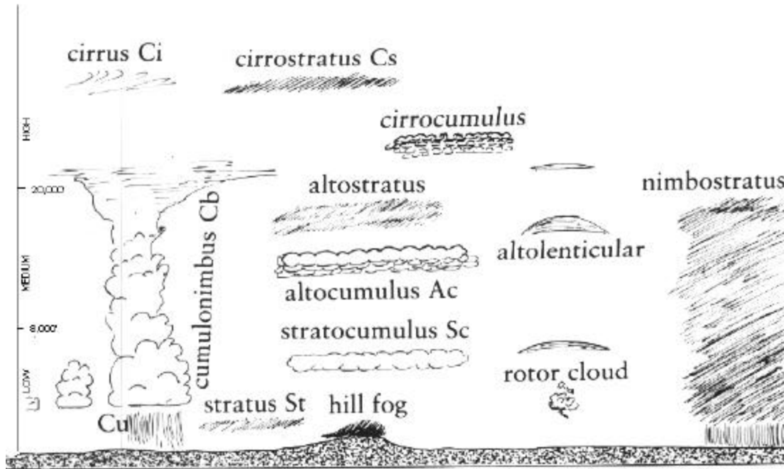
Figure 10 Cloud types
